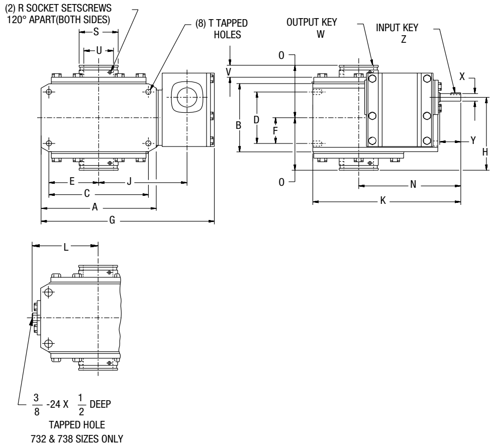
ALL DIMENSIONS IN INCHES
