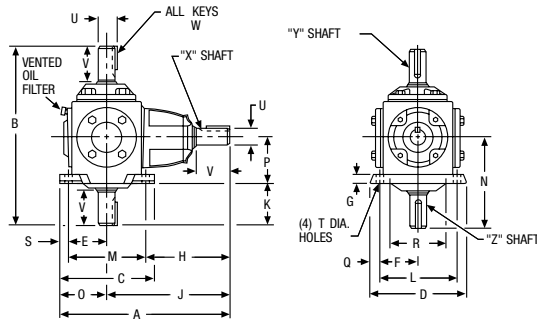
ALL DIMENSIONS IN INCHES
