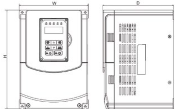
B 10-30 hp, 230V; 15-40 hp, 460V (IP20; NEMA 1)
