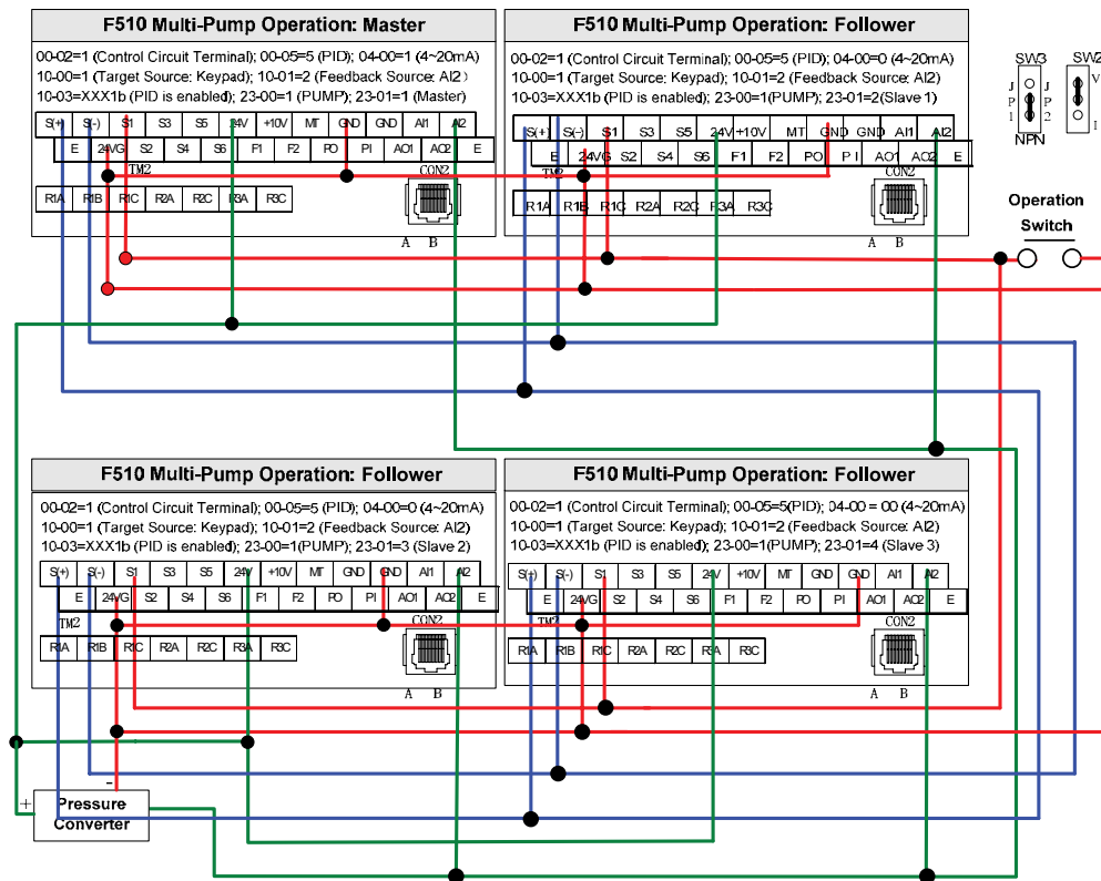
Multi-Pump Wiring Diagram
